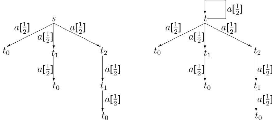
Figure 4: Two states cannot be distinguished without infinite conjunction in FLTSs.
